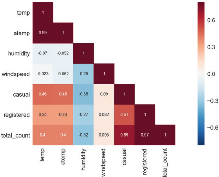
Figure 6-8. Correlational matrix
