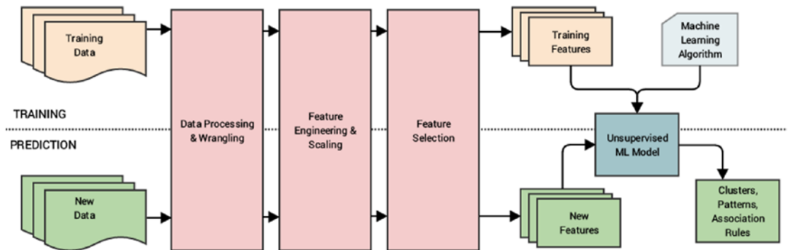
Figure 1-25. Unsupervised Machine Learning pipeline
