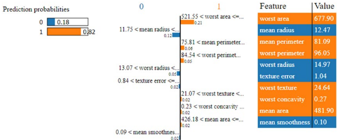
Figure 5-20. Model interpretation for our logistic regression model's prediction for a data point having no cancer (benign)
